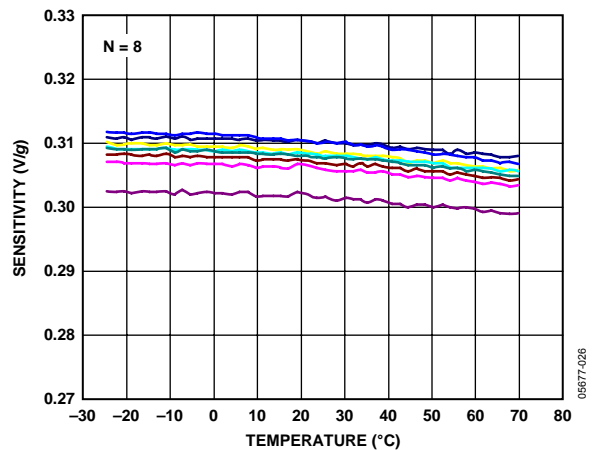
Figure 28. Z-Axis Sensitivity vs. Temperature 8 Parts Soldered to PCB, V_S = 3 V
