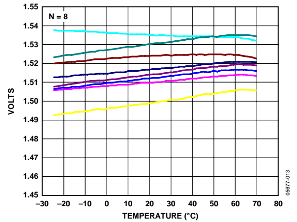
Figure 15. Y-Axis Zero g Bias vs. Temperature—8 Parts Soldered to PCB
