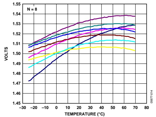
Figure 16. Z-Axis Zero g Bias vs. Temperature—8 Parts Soldered to PCB
