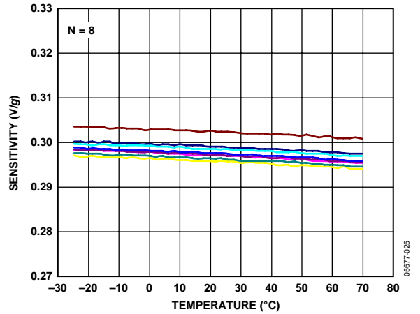
Figure 27. Y-Axis Sensitivity vs. Temperature 8 Parts Soldered to PCB, V_S = 3 V
