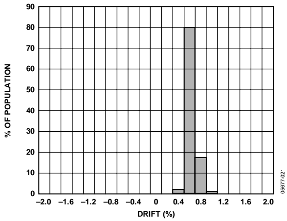
Figure 23. X-Axis Sensitivity Drift Over Temperature, V_S = 3 V
