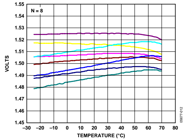
Figure 14. X-Axis Zero g Bias vs. Temperature—8 Parts Soldered to PCB
